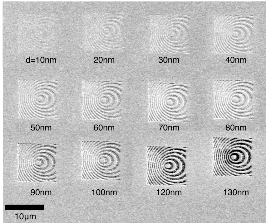
FIGURE 2.6: Composite SEM of samples used to optimize milling depth. Evidence of through-milling begins to appear above 80\ \text{nm} milling depth.
