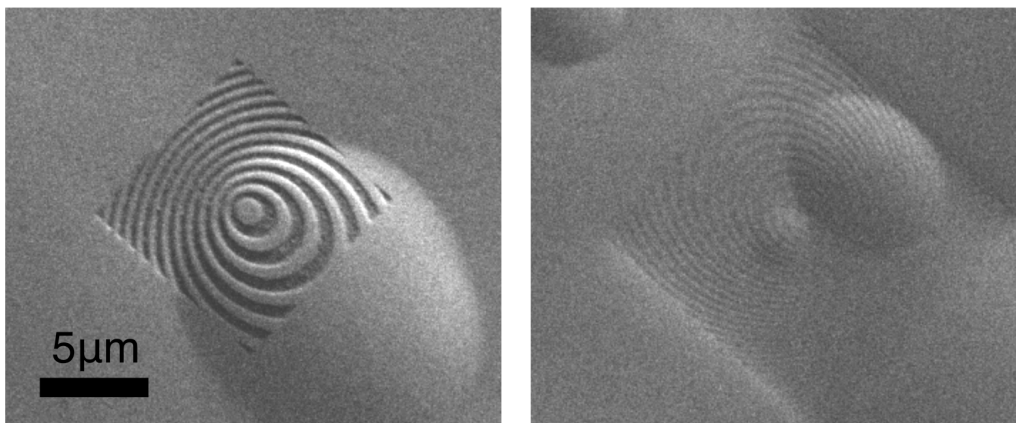
FIGURE 2.5: SEM image of initial holographic metasurface samples fabricated on Silicon Nitride showing delamination of gold film due to heating.
